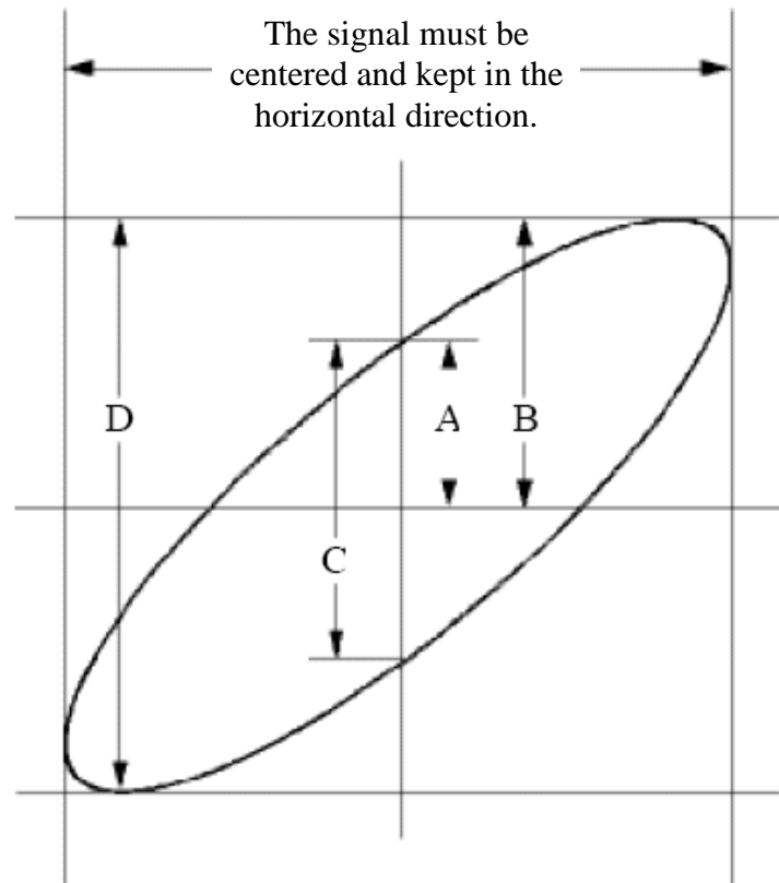
Figure 0-6 Lissajous Graph
